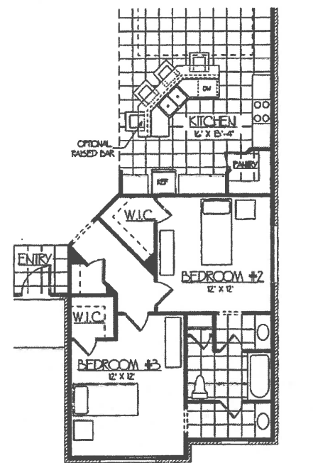
BEDROOM #3 WITH JACK-N-JILL & KITCHEN
